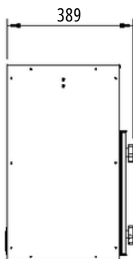
Side Elevation
