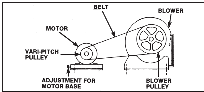
Figure 1 Motor/Blower Assembly
