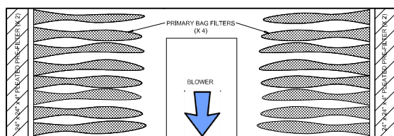
TOP VIEW : CUT-AWAY
