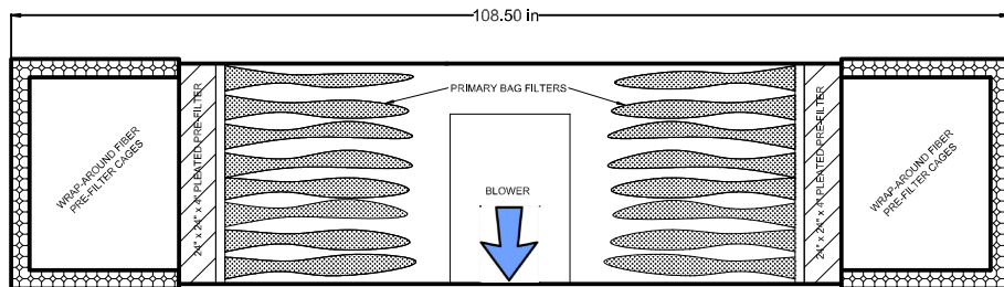
TOP VIEW : CUT-AWAY
